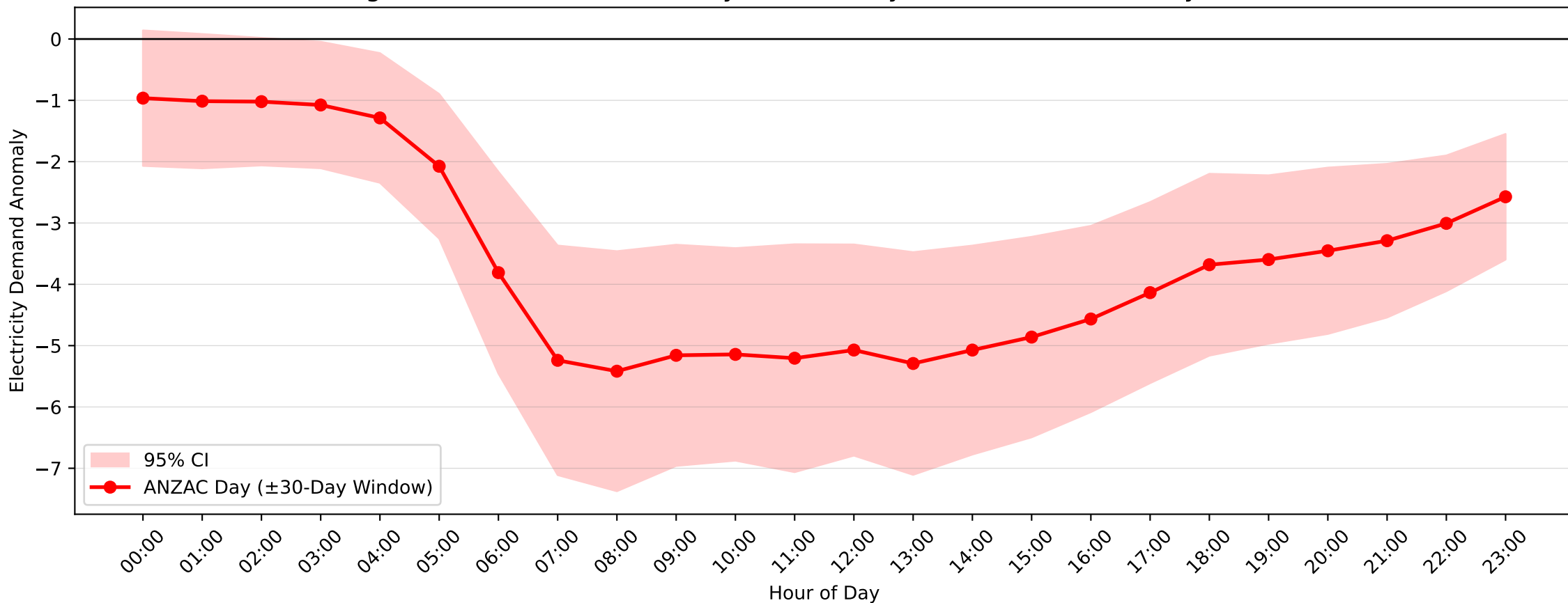
Leightonfield Demand Anomaly: ANZAC Day (2004–2017, \pm 30 -Day Window)
